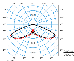
Publisca P1-RB6L/3200-730 4G1S ETDD (CLO initial value) TX301887
