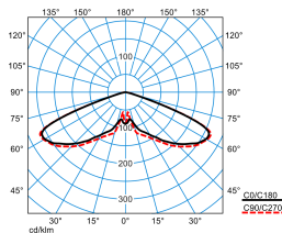
Publisca P1-RB6L/3200-730 4G1S ETDD (CLO end value) TX301407
