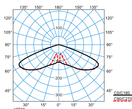
Publisca P1-RB6L/1200-730 2G1S ETDD (CLO initial value) TX301237
