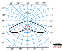
Publisca P1-RB6L/1200-730 2G1S ETDD (CLO end value) TX301261
