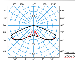
Publisca P1-RB6L/1200-730 2G1S ETDD (CLO initial value)
