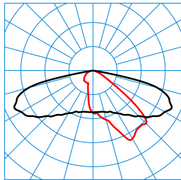
LIQ 50N-AB2L-LR/3200-727 4G1 ET (CLO initial value) TX777726 ■ C0 - C180 ■ C90 - C270 DIN 5040: A30 UTE: 1,00 G DLOR: 100 % ULOR: 0 % CEN Flux Code: 34 71 96 100 100 0 0 0 0
