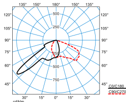
LIQ 70N-FL1L/9100-740 10G1 ET(CLO end value)
