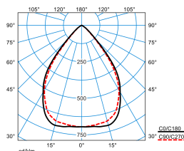
Creavo M73-TS LW19-03 42-8TW ETBLE-S 01 (DSU)
