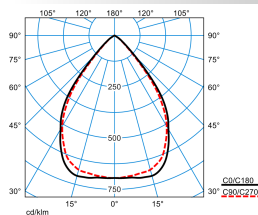
Creavo M73-TS LW19-03 42-8TW ETBLE-S 01 (DWW)
