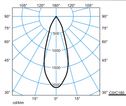
Can G2 3P RF-FL 30-BC M49 ETBLE 01
