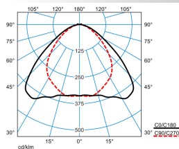
ELINE HE+ LVW100 830 L225 1 20
