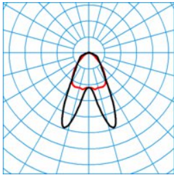
ELINE FL HE+ LDAN180 865 L225 1 20
