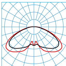
Publisca P1W-RBT-LRA/3800-740 6G1S ET (CLO initial value) TX300817 ■ C0 - C180 ■ C90 - C270 DIN 5040: A20 UTE: 0.98 l + 0.02 T DLOR: 98 % ULOR: 2 % CEN Flux Code: 26 63 91 98 100 0 0 0 2
