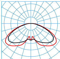
Publisca P1W-RBT-LRA/3800-740 6G1S ET (CLO end value) TX300453 ■ C0 - C180 ■ C90 - C270 DIN 5040: A20 UTE: 0.98 l + 0.02 T DLOR: 98 % ULOR: 2 % CEN Flux Code: 26 63 91 98 100 0 0 0 2
