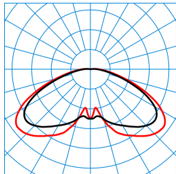
Publisca P1W-RBT-LRA/3800-740 6G1S TX053590 ■ C0 - C180 ■ C90 - C270 DIN 5040: A20 UTE: 0.98 l + 0.02 T DLOR: 98 % ULOR: 2 % CEN Flux Code: 26 63 91 98 100 0 0 0 2
