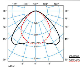
ELINE LVW160 840 L225 1 20
