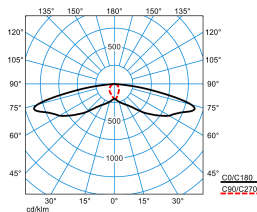
LIQ 50N-SB3L-LRA/1350-722 2G1 ETDD (CLO initial value) TX779866
