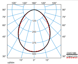
SFlow D2-L MRWD LED4000-830 ETDD 01 TX770114
