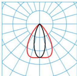
ELINE FL HE+ LVN120 840 L225 1 20
