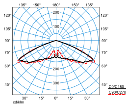
Publisca P1W-RB6L-LR/1200-730 2G1S
