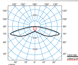
LIQ 50N-SB3L-SLR1/2200-740 2G1 ET (CLO initial value)
