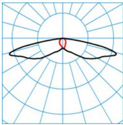
Jovie 50-SB3L-2-13-730-CLO-B
