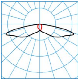
Jovie 50-SB3L-2-13-730-CLO-E
