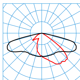
LIQ 70N-AB7L-LR/10000-727 12G1 ET(CLO initial value) TX277808 ■ C0 - C180 ■ C90 - C270 DIN 5040: A30 UTE: 1,00 E DLOR: 100 % ULOR: 0 % CEN Flux Code: 39 76 98 100 100
