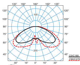
Publisca P1W-RBT-LRA/2600-740 3G1S ET (CLO initial value) TX301161 DIN 5040: A20 UTE: 0.99 I + 0.01 T DLOR: 99 % ULOR: 1 % CEN Flux Code: 26 63 91 99 100 0 0 0 1
