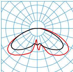
Publisca P1W-RBT-LRA/2600-740 3G1S ET (CLO end value) TX300214 ■ C0 - C180 ■ C90 - C270 DIN 5040: A20 UTE: 0.99 l + 0.01 T DLOR: 99 % ULOR: 1 % CEN Flux Code: 26 63 91 99 100 0 0 0 1
