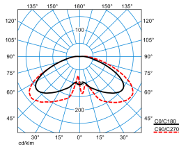
Publisca P1W-RBT-LRA/2600-740 3G1S
