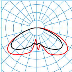
Publisca P1W-RBT-LRA/2600-740 3G1S TX053586 ■ C0 - C180 ■ C90 - C270 DIN 5040: A20 UTE: 0.99 l + 0.01 T DLOR: 99 % ULOR: 1 % CEN Flux Code: 26 63 91 99 100 0 0 0 1
