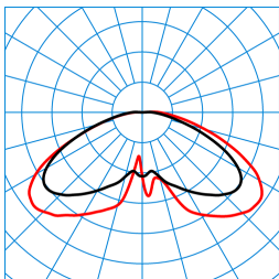
Publisca P1W-RBT-LRA/2600-740 3G1S ET (CLO initial value) TX301161 ■ C0 - C180 ■ C90 - C270 DIN 5040: A20 UTE: 0.99 l + 0.01 T DLOR: 99 % ULOR: 1 % CEN Flux Code: 26 63 91 99 100 0 0 0 1
