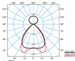
SFlow H2-L MRX LED6400-8TW ETDD8 01 (DSU) TX877179
