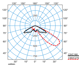
LnPlus 60-AM19L/20000-730 24G1 ETDD (CLO initial value) TX377162
