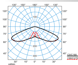
Publisca P1-RB6L/1350-730 2G1S ETDD (CLO initial value)
