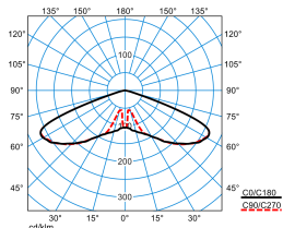
Publisca P2-RB6L/1100-740 2G1S ETDD (CLO end value)
