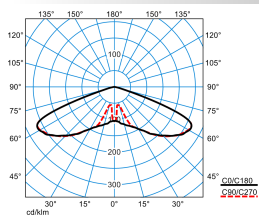
Publisca P2-RB6L/1100-740 2G1S ETDD (CLO initial value)
