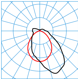
TugraHE 15 PAW 30-93/16ML-840 ET PC 23 (stage 12) TX779199 C0 - C180 C90 - C270
