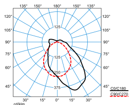
TugraHE 15 PAW 30-93/16ML-840 ET PC 23 (stage 1)
