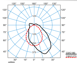
TugraHE 15 PAW 30-93/16ML-840 ET PC 23 (stage 0)
