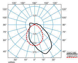
TugraHE 15 PAW 30-93/16ML-840 ET PC 23 (stage 2)
