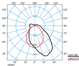
TugraHE 15 PAW 30-93/16ML-840 ET PC 23 (stage 5)
