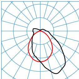
TugraHE 15 PAW 30-93/16ML-840 ET PC 23 (stage 13) TX779205 C0 - C180 C90 - C270
