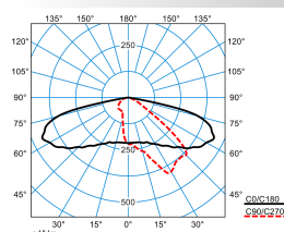
LIQ 50N-AB2L-SLR2/4200-722 4G1 ET (CLO initial value)
