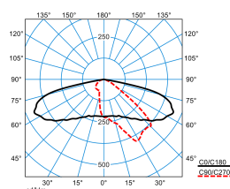
LIQ 50N-AB2L-SLR2/4200-722 4G1 ET (CLO end value)
