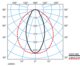
Nextrema G3 TB 80-840 ET +LV TWP PC TX768235
