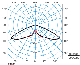
Publisca P1W-RB6L-LR/3800-730 6G1S
