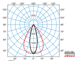
ELINE LEN55-140 ML 840 L225 4 50
