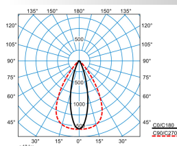
ELINE LEN55-140 ML 840 L225 0 50
