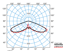
Publisca P1-RB6L/2600-740 3G1S ETDD (CLO initial value)
