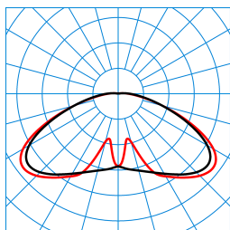
Publisca P1W-RBT-LRA/1500-730 2G1S ET (CLO end value) TX300270 ■ C0 - C180 ■ C90 - C270 DIN 5040: A20 UTE: 0.97 l + 0.03 T DLOR: 97 % ULOR: 3 % CEN Flux Code: 26 63 91 97 100 4 16 28 3
