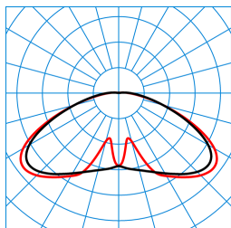
Publisca P1W-RBT-LRA/1500-730 2G1S TX053579 ■ C0 - C180 ■ C90 - C270 DIN 5040: A20 UTE: 0.97 l + 0.03 T DLOR: 97 % ULOR: 3 % CEN Flux Code: 26 63 91 97 100 4 16 28 3
