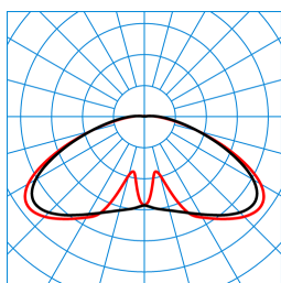
Publisca P1W-RBT-LRA/1500-730 2G1S ET (CLO initial value) TX301593 ■ C0 - C180 ■ C90 - C270 DIN 5040: A20 UTE: 0.97 l + 0.03 T DLOR: 97 % ULOR: 3 % CEN Flux Code: 26 63 91 97 100 4 16 28 3
