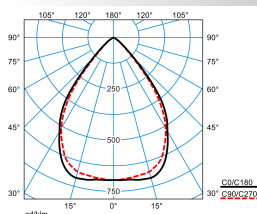
Creavo M39 LW19-03 53-8TW ETBLE 01 (DWW)
