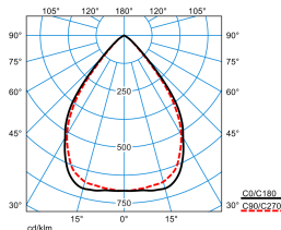
Creavo M39 LW19-03 53-8TW ETBLE 01 (DCW)
