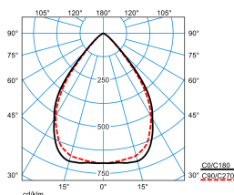
Creavo M39 LW19-03 53-8TW ETBLE 01 (DSU)
