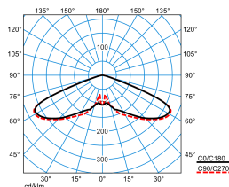
Publisca P2-RB6L/4200-730 6G1S ETDD (CLO end value)
