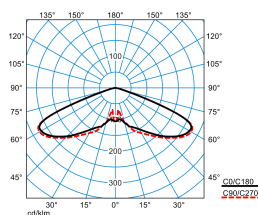
Publisca P2-RB6L/4200-730 6G1S
