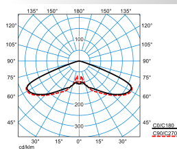
Publisca P2-RB6L/4200-730 6G1S ETDD (CLO initial value)
