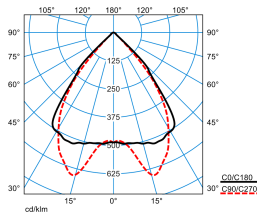
SFlow D1-L MRX LED3200-840 ETDD 03 TX769895
