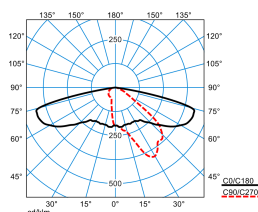
9301K AB2L-SLR3/4600-740 8G3 ET(CLO end value)
