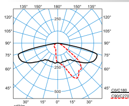
9301K AB2L-SLR3/4600-740 8G3 ET(CLO initial value)
