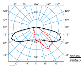
LIQ 50N-AB2L-LR-SLR2/6800-727 6G1 ET (CLO end value)
