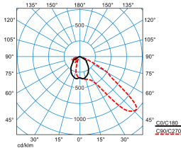
Jovie 50I-AM2L-MLLR/16-42-730 4G1 ETDD (CLO end value) TX775192
