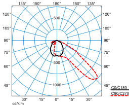
Jovie 50I-AM2L-MLLR/16-42-730 4G1 ETDD (CLO initial value) TX775193
