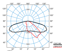
LIQ 50N-AB2L-LR-SLR2/4200-740 4G1 ET (CLO end value)
