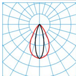
ELINE FL LEN100 840 L225 1 20
