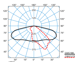
LIQ50N-AB2L6S3-34-7TW-ET-CAB-26 (DSU-CLO initial value)
