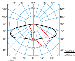
LIQ50N-AB2L6S3-34-7TW-ET-CAB-26 (DCW-CLO end value)
