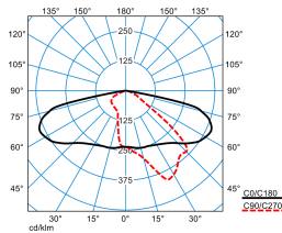
LIQ50N-AB2L6S3-34-7TW-ET-CAB-26 (DCW-CLO initial value)
