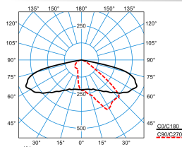
LIQ 50N-AB2L-LR/6200-727 6G1 ET (CLO initial value)
