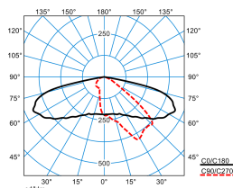
LIQ 50N-AB2L-LR/6200-727 6G1 ET (CLO end value)
