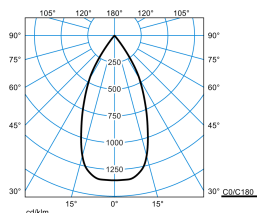
E-Line PRO 78 BV G2 RF-WFL 50-830 M33 ETDD 05 05
