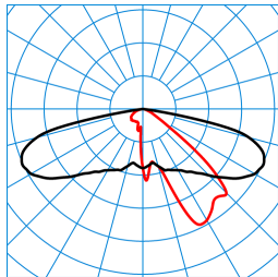
Publisca P2-AB2L/2400-740 3G1S ETDD (CLO initial value) TX301662 ■ C0 - C180 ■ C90 - C270 DIN 5040: A30 UTE: 1,00 l DLOR: 100 % ULOR: 0 % CEN Flux Code: 34 71 96 100 100
