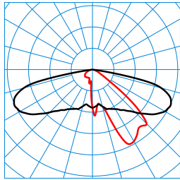
Publisca P2-AB2L/2400-740 3G1S ETDD (CLO end value) TX301668 ■ C0 - C180 ■ C90 - C270 DIN 5040: A30 UTE: 1,00 l DLOR: 100 % ULOR: 0 % CEN Flux Code: 34 71 96 100 100
