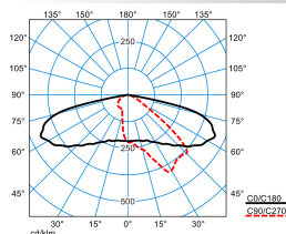
LIQ 50N-AB2L-LRA/4600-727 6G1 ETDD (CLO initial value)
