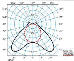
AragF 15 PVW 44-840 ETDD +HFS PC TX782394
