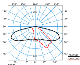
LIQ 50N-AB2L-LR/3500-727 4G1 ET (CLO initial value) TX777781
