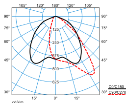
Jovie 70I-AM3L-MLLR/75-150-740 12G1 ETDD (CLO end value)
