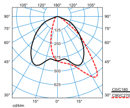
Jovie 70I-AM3L-MLLR/75-150-740 12G1 ETDD (CLO initial value)
