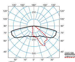
9301K AB2L-SLR3/2600-730 4G3 ET(CLO end value)
