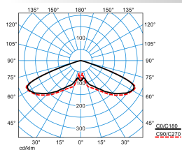
Publisca P1-RB6L/2900-730 4G1S ETDD (CLO initial value)
