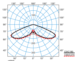
Publisca P1-RB6L/2900-730 4G1S ETDD (CLO end value)
