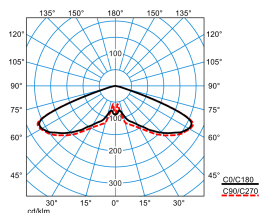
Publisca P1-RB6L/2900-730 4G1S
