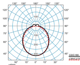
ELINE DSL35-100 ML 865 L150 0 50
