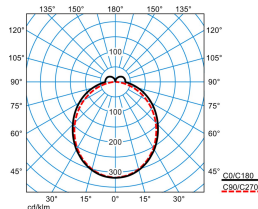
ELINE DSL35-100 ML 865 L150 4 50
