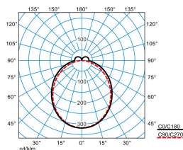
ELINE DSL35-100 ML 865 L150 2 50
