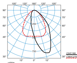
ELINE LAN55-140 ML 865 L225 4 50
