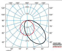
Sanesca W2 5000 ETDD8/ET 840 01 (DWW) (reading light) TX874751
