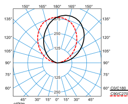
Sanesca W2 5000 ETDD8/ET 840 01 (DSU) (room light) TX874750
