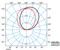
Sanesca W2 5000 ETDD8/ET 840 01 (DWW) (room light) TX874752
