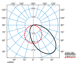
Sanesca W2 5000 ETDD8/ET 840 01 (DSU) (reading light) TX874749
